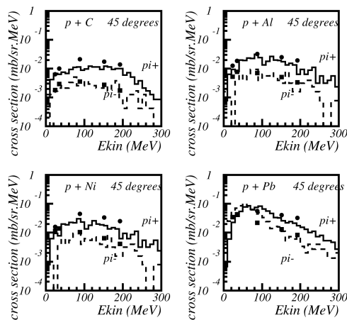
Fig. 26.13: Double differential cross-section for pions produced at 45^\circ in proton scattering off various materials. Proton incident energy was 597 MeV in each case. The points are data, the histogram is Binary Cascade prediction.
