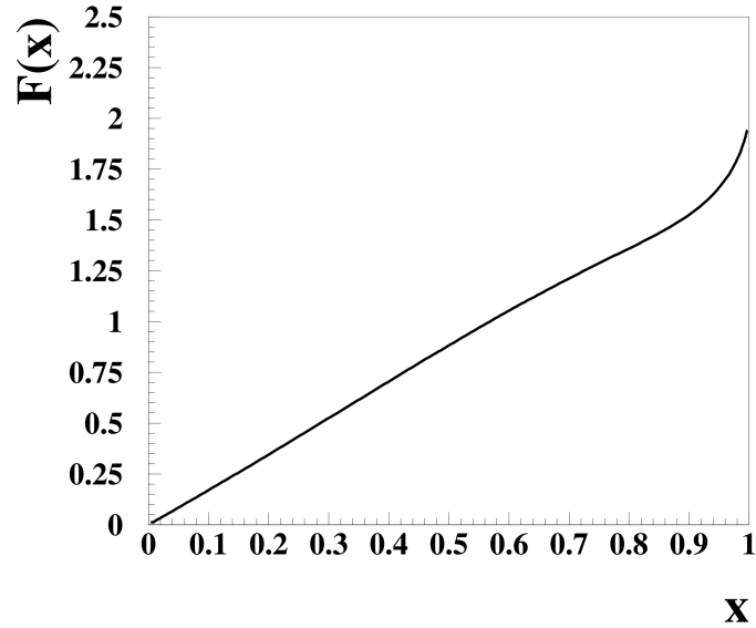
Fig. 5.1: Graph of F(x) ((5.2)).
