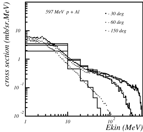
Fig. 26.3: Double differential cross-section for neutrons produced in proton scattering off Aluminum. Proton incident energy was 597 MeV. The points are data, the histogram is Binary Cascade prediction.
