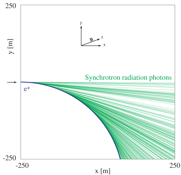
Fig. 15.4: GEANT4 display. 10 GeV e^+ moving initially in x-direction, bends downwards on a circular path by a 0.1T magnetic field in z-direction.
