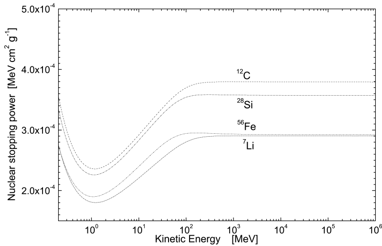
Fig. 9.5: In \text{MeVcm}^2/\text{g} , nuclear stopping powers in {}^7\text{Li} , {}^{12}\text{C} , {}^{28}\text{Si} and {}^{56}\text{Fe} calculated from Eq.(9.75) and divided by the density of the material as a function of the kinetic energy of electrons from 200 keV up to 1 TeV.
