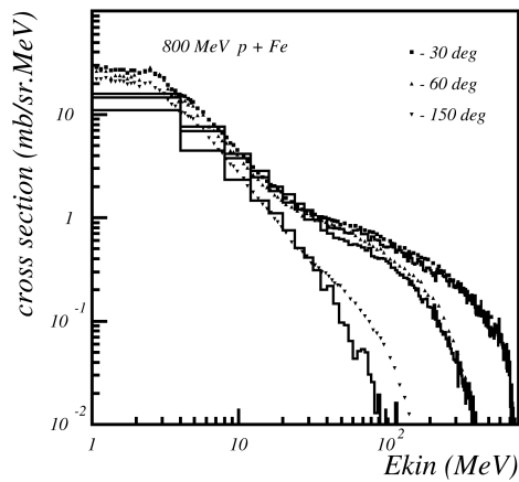
Fig. 26.8: Double differential cross-section for neutrons produced in proton scattering off Iron. Proton incident energy was 800 MeV. The points are data, the histogram is Binary Cascade prediction.
