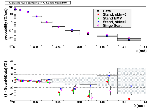
Fig. 9.1: Scattering of muons off 1.5 mm aluminum foil: data [ea106] - black squares; simulation - colored markers corresponding different options of multiple scattering and single scattering model; in the bottom plot - relative difference between the simulation and the data in percents; hashed area demonstrates one standard deviation of the data.
