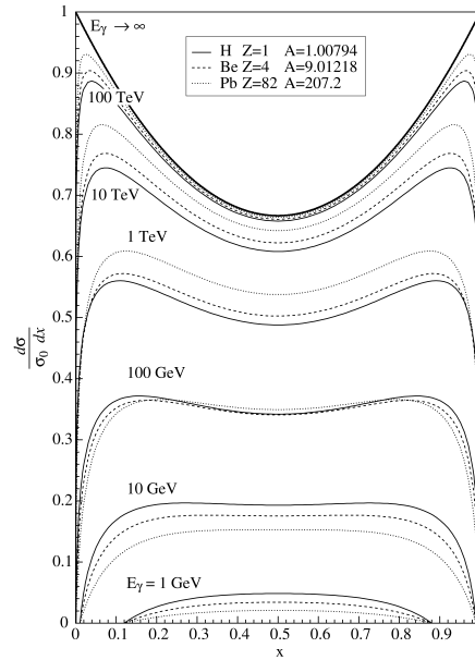
Fig. 7.3: Normalized differential cross section for pair production as a function of x , the energy fraction of the photon energy carried by one of the leptons in the pair. The function is shown for three different elements, hydrogen, beryllium and lead, and for a wide range of photon energies.
