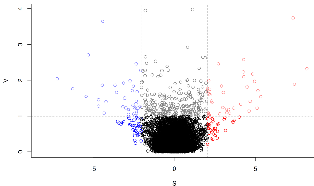
Figure 2: SV-plot produced from a GEVAQuantiles object using the geva.quantiles function with default parameters.
