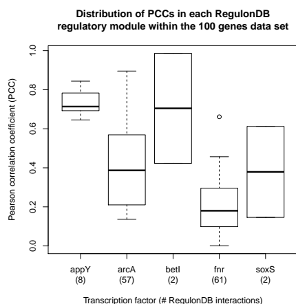
Figure 1: Distribution of Pearson correlation coefficients (PCCs) calculated from the Covert et al. (2004) oxygen deprivation data between genes forming RegulonDB interactions
