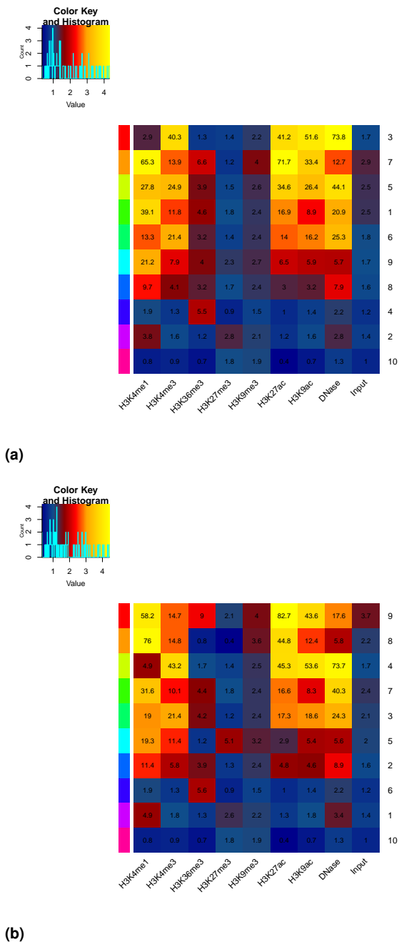
Figure 1: Mean read counts of the (a) 'NegativeBinomial' and (b) 'PoissonLogNormal' state annotation
