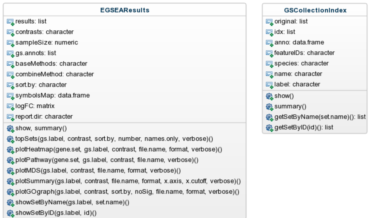
Figure 1: The S4 classes and methods of EGSEA .
