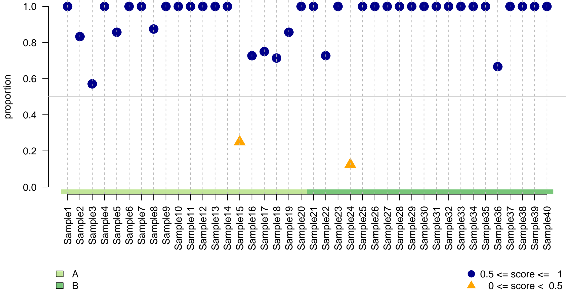
Freq. of being correctly classified (svm, 7 feat.)
