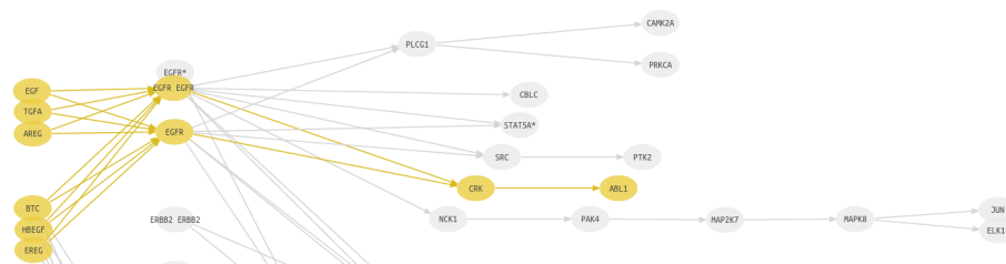
Figure 7: Effector subpathway depicted in yellow
