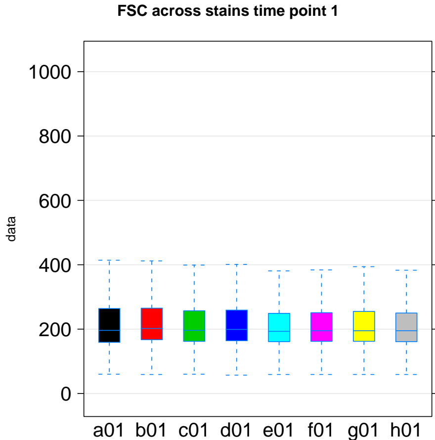
Figure 3: boxplot.FCS: Boxplot of the Forward Scatter parameter of the different stains at different 4 different time points (flowcyt.fluors FCS R object)
