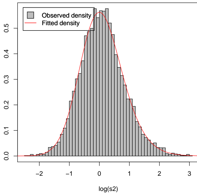
Figure 5: Comparing the fitted distribution for \log(s^2) with the observed data from the ApoAI knockout experiment.
