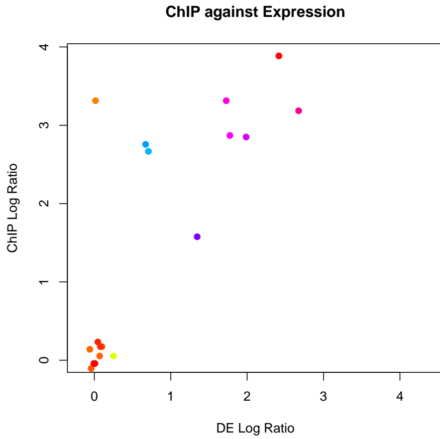
Figure 2: Output from plotMM(Rcade) .
