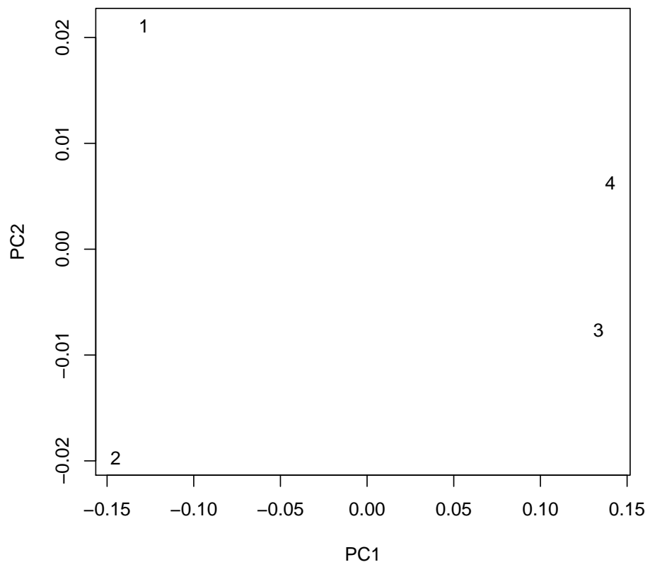
Figure 1: Output from plotPCA(Rcade) .
