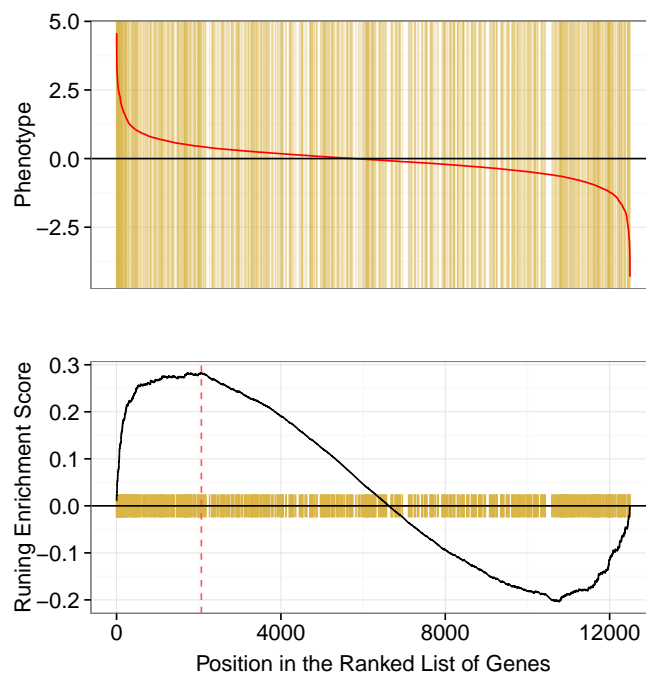
Figure 5: gseaplot example.
