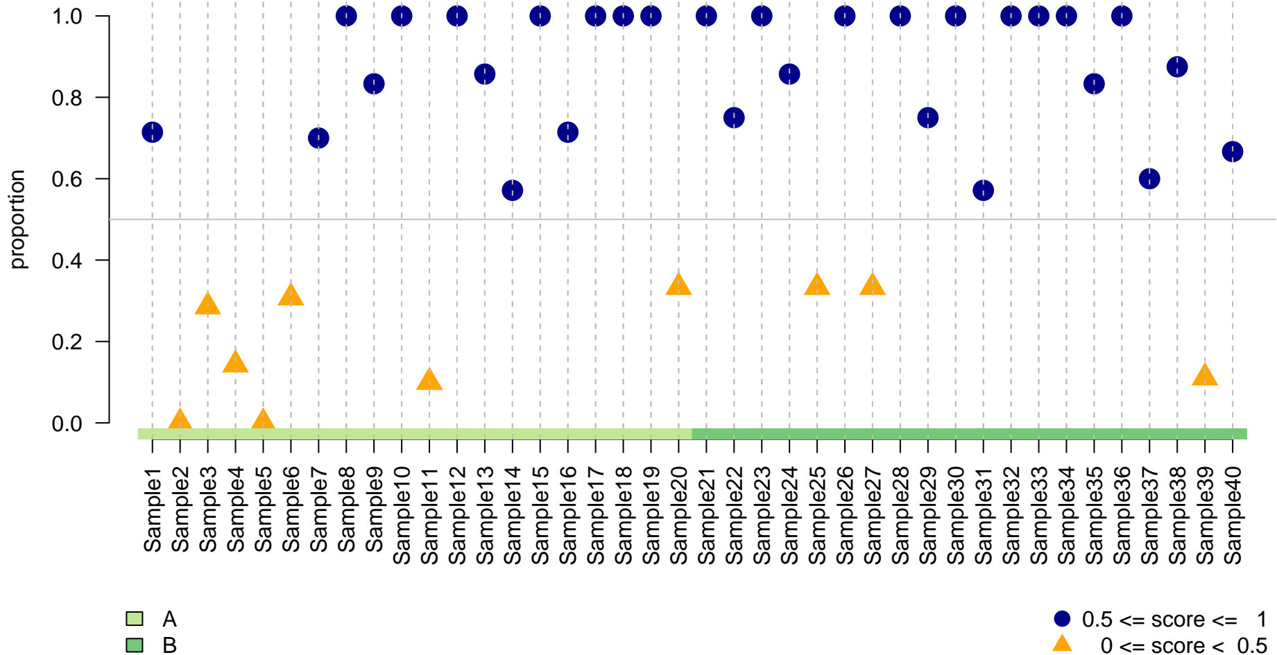
Freq. of being correctly classified (randomForest, 15 feat.)
