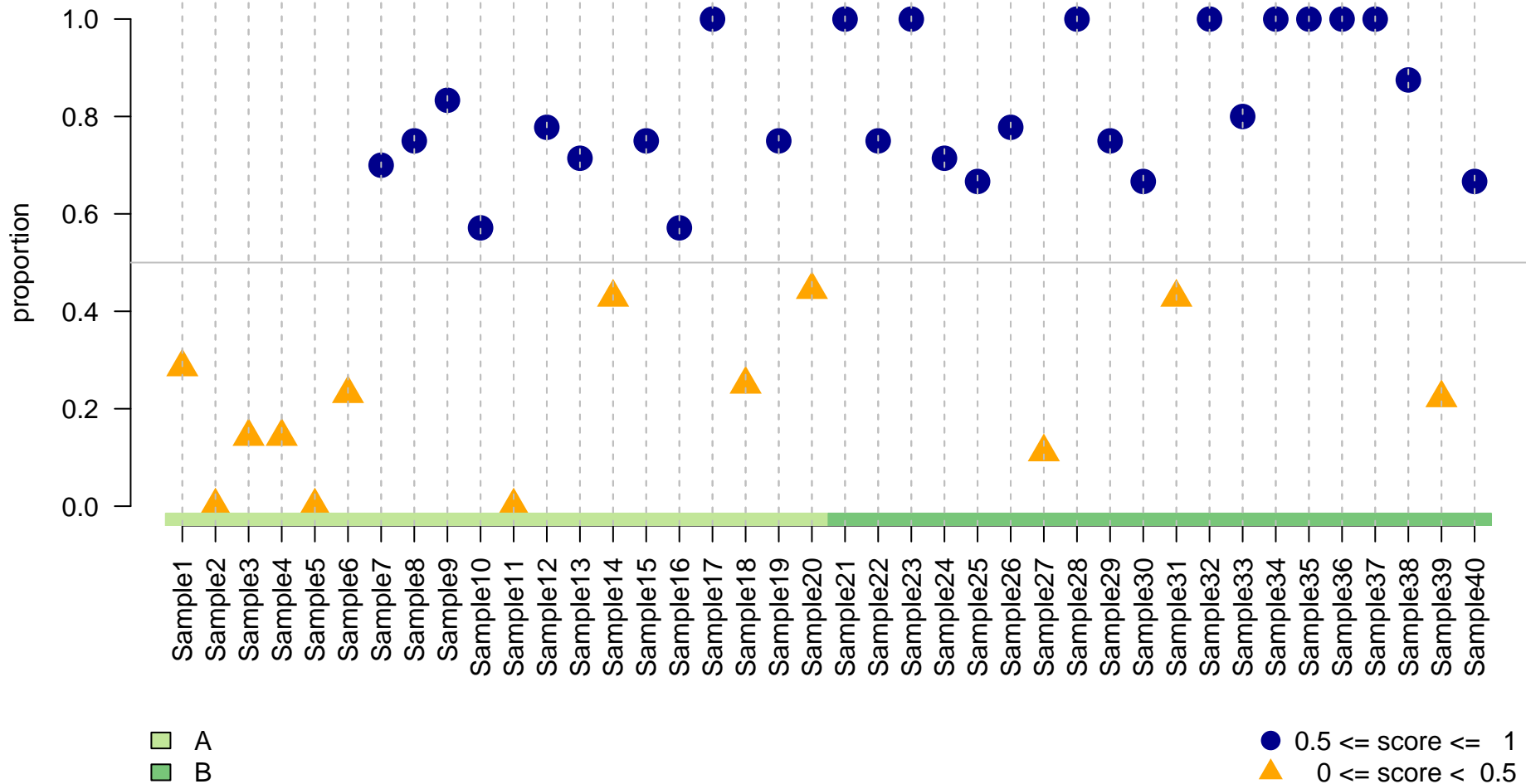
Freq. of being correctly classified (pam, 2 feat.)
