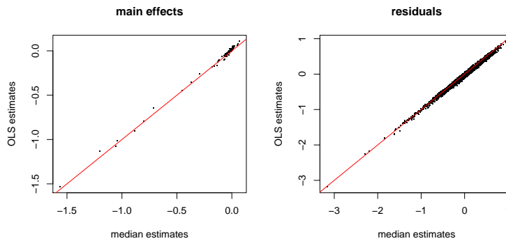
Figure 18: Effect fitted by lmmain and estmodel .
