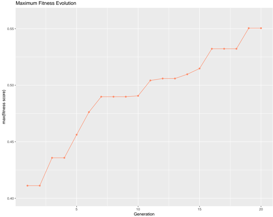
Figure 1: Fitness Evolution plot The plot shows the evolution of the maximum fitness across the generations
