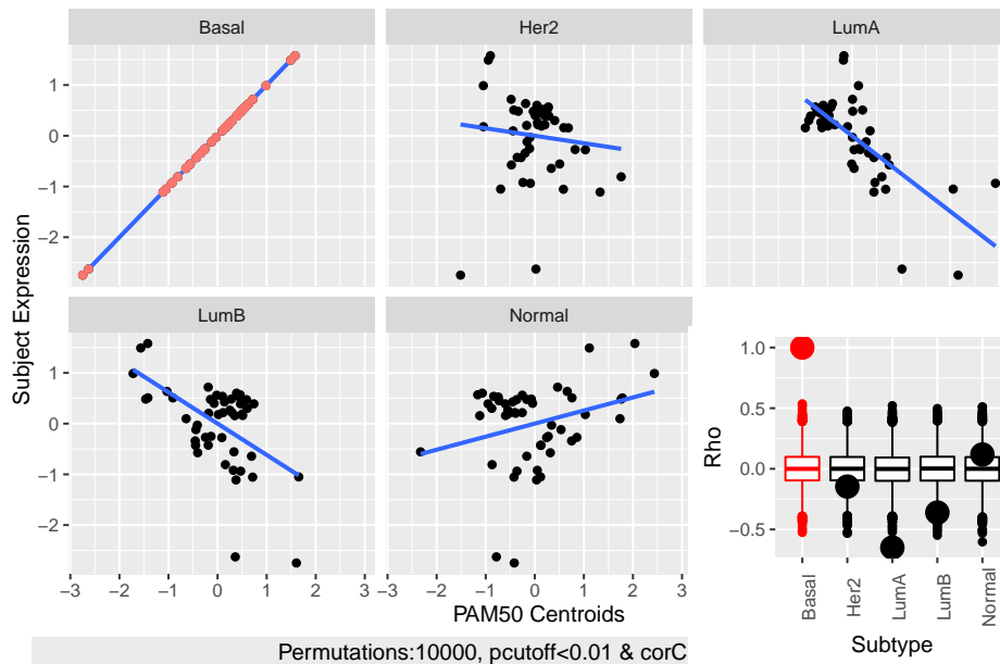
Figure 2: PAM50 permutation subject report for genefu 's "Basal" intrinsic gene profile (IGP). The top table summarizes the results for the i -th subject, i. e., the correlation, p-value and false discovery rate (fdr) obtained for each IGP. In addition, scatter plots of the observed subject gene profiles against the IGP with the linear regression line (in blue). Red color indicates the assigned subtype. Finally, a boxplot for each IGP null permuted correlation distribution and big dots to represent the un-permuted observed correlations.
