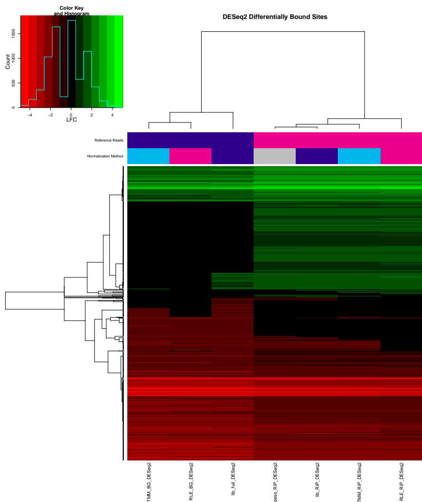
Figure 27: Clustering heatmap of differentially bound sites from DESeq2 analyses using various normalization and reference read methods
