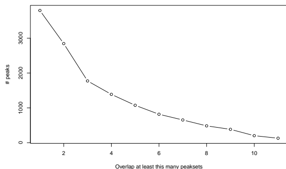
Figure 35: Overlap rate plot. Shows how the number of overlapping peaks decreases as the overlap criteria becomes more stringent. X axis shows the number of peaksets in which the site is identified, while the Y axis shows the number of overlapping sites. Generated by plotting the result of: dba.overlap(tamoxifen,mode=DBA_OLAP_RATE)
