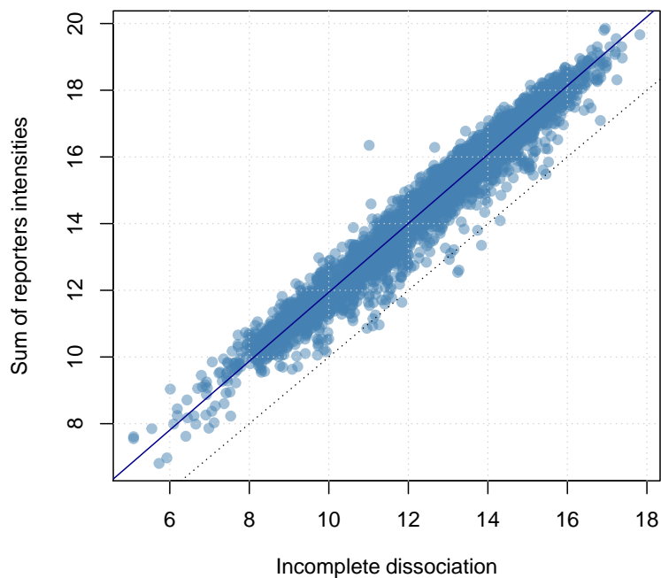
Figure 6: Incomplete dissociation.
